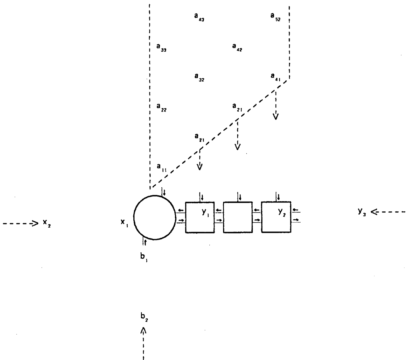
Fig. 2.6.2. The linearly connected network for solving the linear system shown in Fig. 2.6.1.
