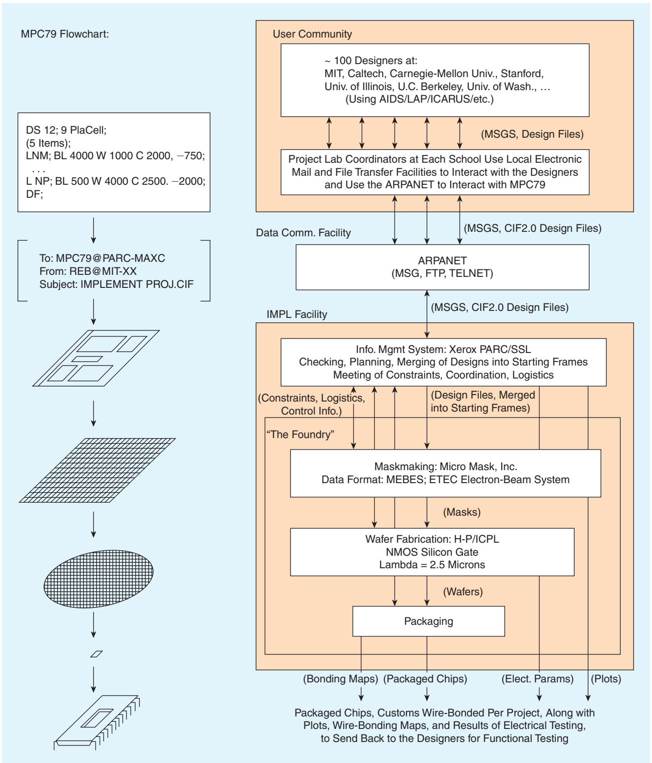
FIGURE 11: Flowchart of events for MPC79.
